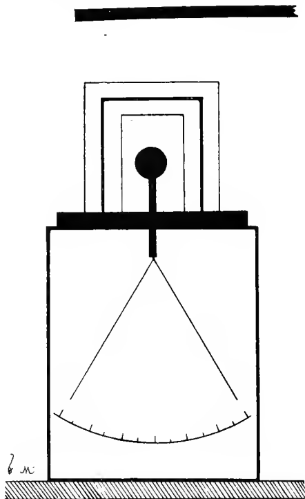
Fig. 9.—Passage of lines of force through three concentric metallic screens of varying thickness surrounding the ball of an electro-scope. Under the influence of a glass or resin rod rubbed and brought close to the instrument, the gold leaves immediately diverge.
